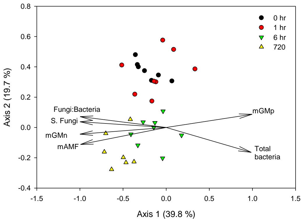
Fig. 2.18. Distance based redundancy analysis (db RDA) plot derived from fatty acid profiles from samples collected in corn stubble residue from no-till treatment at pre- (0 hrs) and up to 720 hrs (30 days) post-management. Pre are black circles, 1 hr is red circles, 6 hrs are green triangles, and 720 hrs are gold triangles. Vectors in the bi-plot overlay were constructed from a matrix containing taxonomic groups. (mGMp = Gram positive bacteria; mGMn = Gram negative bacteria; mAMF = Arbuscular mycorrhizal fungi; S. Fungi = Saprophytic Fungi)
