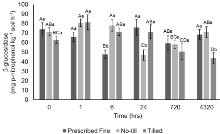
Fig. 2.12. \beta -glucosidase activity in samples from prescribed fire, no-till, and conventionally tilled treatments pre- (0 hrs) and up to 4320 hrs (6 months) post-management of corn residue. Different uppercase letters indicate significant differences within treatment over time. Different lowercase letters indicate significant differences within time between treatments. ( \alpha=0.05 )
