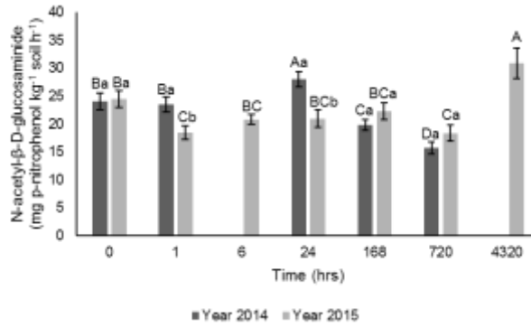
Fig. 2.14. N-acetyl- \beta -D-glucosaminidase (NAGase) activity in samples collected year 2014 and 2015 from prescribed fire, no-till, and conventionally tilled treatments pre- (0 hrs) and up to 4320 hrs (6 months) post-management of wheat residue. Different uppercase letters indicate significant differences within years over time. Different lowercase letters indicate significant differences within time between years. ( \alpha=0.05 )
