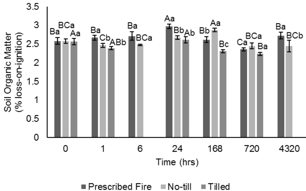
Fig. 2.1. Soil organic matter concentration in samples from prescribed fire, no-till, and conventionally tilled treatments pre- (0 hrs) and up to 4320 hrs (6 months) post-management of wheat residue. Different uppercase letters indicate significant differences within treatments over time. Different lowercase letters indicate significant differences within time between treatments. ( \alpha=0.05 )
