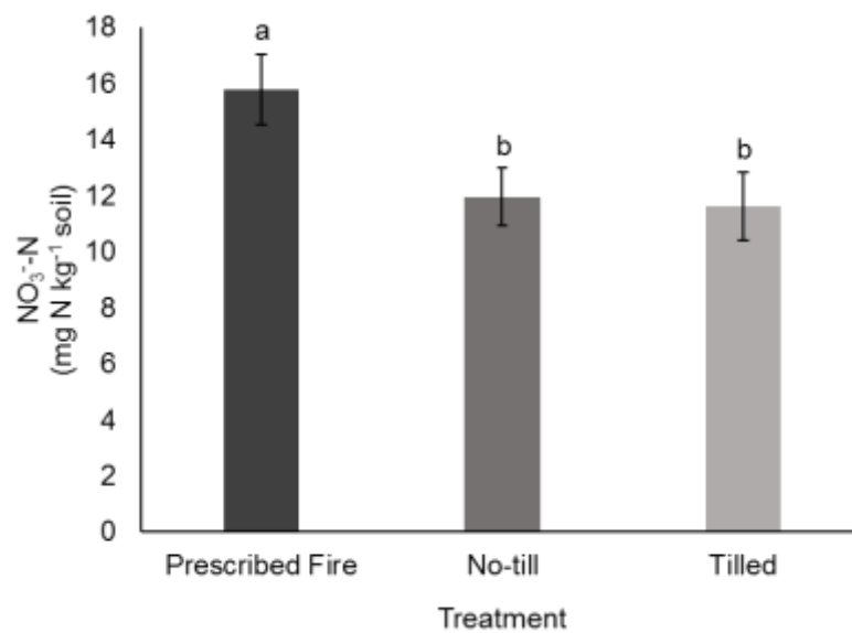
Fig. 2.4. Nitrate-N ( \text{NO}_3^- -N) concentration in samples averaged over time from pre- (0 hrs) to 4320 hrs (6 months) post-management in prescribed fire, no-till, and conventionally tilled treatments in wheat residue. Different lowercase letters indicate significant differences within time between treatments. ( \alpha=0.05 )
