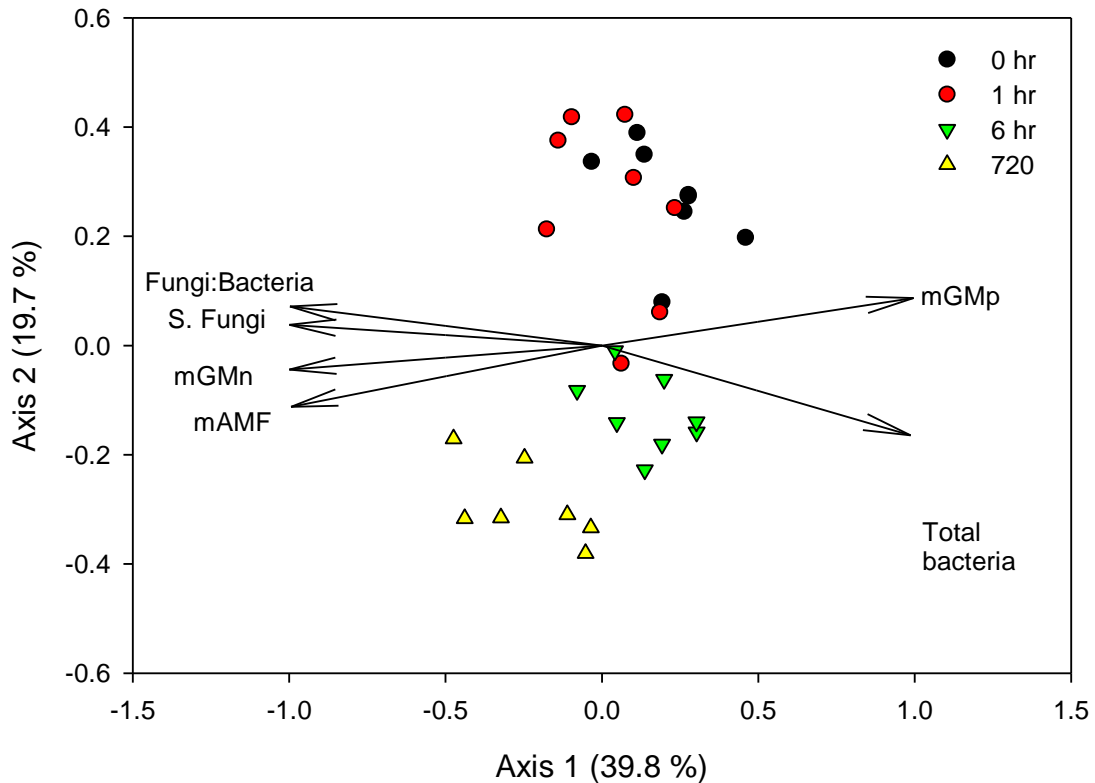
Fig. 2.19. Distance based redundancy analysis (db RDA) plot derived from fatty acid profiles from samples collected in corn stubble residue from tilled treatment at pre- (0 hrs) and up to 720 hrs (30 days) post-management. Pre are black circles, 1 hr is red circles, 6 hrs are green triangles, and 720 hrs are gold triangles. Vectors in the bi-plot overlay were constructed from a matrix containing taxonomic groups. (mGMp = Gram positive bacteria; mGMn = Gram negative bacteria; mAMF = Arbuscular mycorrhizal fungi; S. Fungi = Saprophytic Fungi)
