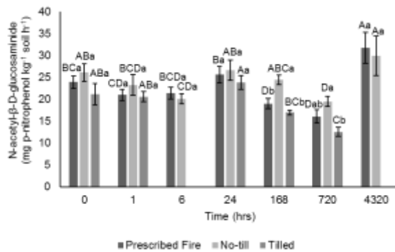
Fig. 2.13. N-acetyl- \beta -D-glucosaminidase (NAGase) activity in samples from prescribed fire, no-till, and conventionally tilled treatments pre- (0 hrs) and up to 4320 hrs (6 months) post-management of wheat residue. Different uppercase letters indicate significant differences within treatments over time. Different lowercase letters indicate significant differences within time between treatments. ( \alpha=0.05 )
