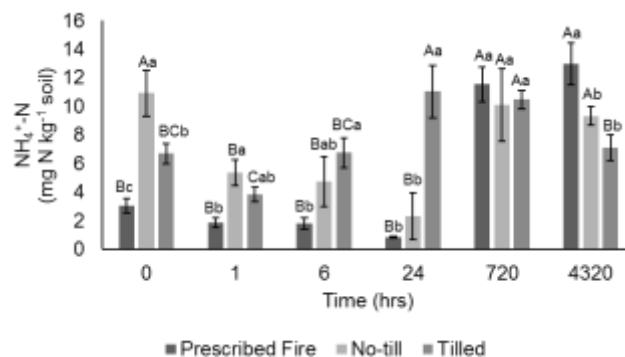
Fig. 2.9. Ammonium-N ( \text{NH}_4^+\text{-N} ) concentration in samples from prescribed fire, no-till, and conventionally tilled treatments pre- (0 hrs) and up to 4320 hrs (6 months) post-management of corn residue. Different uppercase letters indicate significant differences within treatment over time. Different lowercase letters indicate significant differences within time between treatments. ( \alpha=0.05 )
