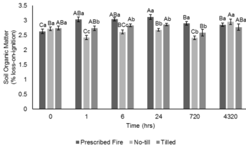
Fig. 2.3. Soil organic matter concentration in samples from prescribed fire, no-till, and conventionally tilled treatments pre- (0 hrs) and up to 4320 hrs (6 months) post-management of corn residue. Different uppercase letters indicate significant differences within treatment over time. Different lowercase letters indicate significant differences within time between treatments. ( \alpha=0.05 )
