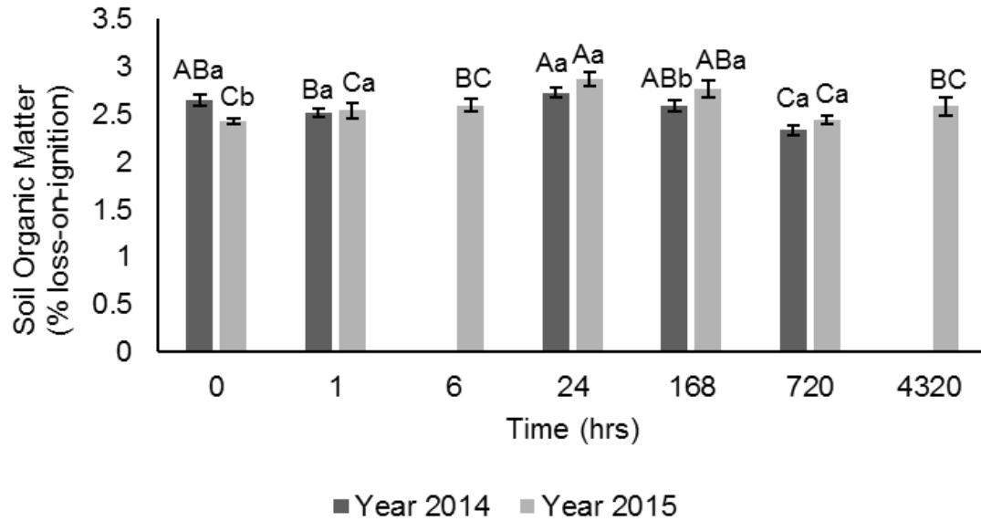
Fig. 2.2. Soil organic matter concentration in samples collected year 2014 and 2015 from prescribed fire, no-till, and conventionally tilled treatments pre- (0 hrs) and up to 4320 hrs (6 months) post-management of wheat residue. Different uppercase letters indicate significant differences within years over time. Different lowercase letters indicate significant differences within time between years. ( \alpha=0.05 )
