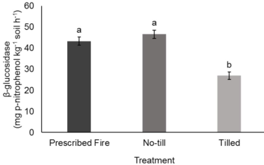
Fig. 2.10. \beta -glucosidase activity in samples averaged over time from pre- (0 hrs) to 4320 hrs (6 months) post-management in prescribed fire, no-till, and conventionally tilled treatments in wheat residue. Different lowercase letters indicate significant differences within time between treatments. ( \alpha=0.05 )
