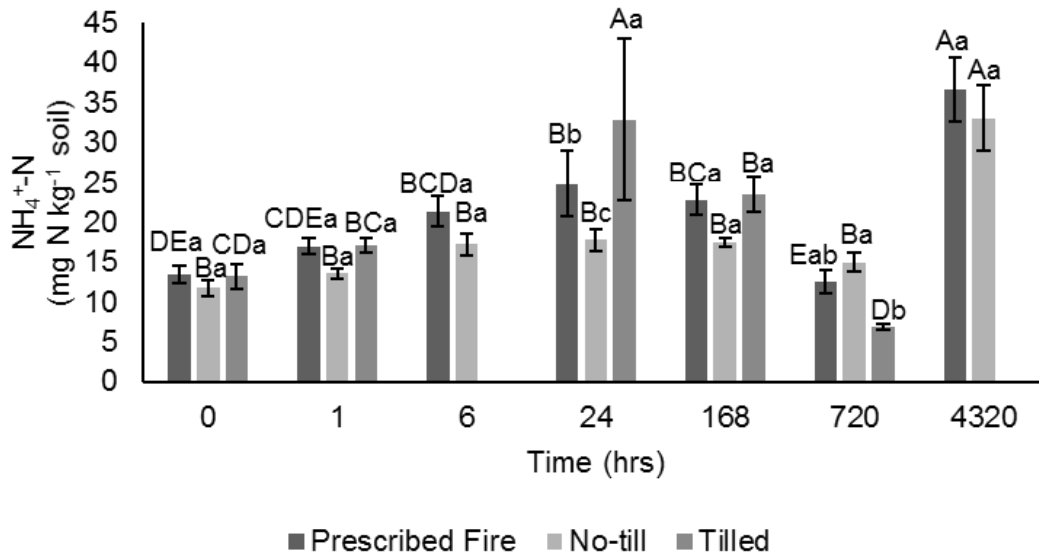
Fig. 2.6. Ammonium-N ( \text{NH}_4^+\text{-N} ) concentration in samples collected year 2014 and 2015 from prescribed fire, no-till, and conventionally tilled treatments pre- (0 hrs) and up to 4320 hrs (6 months) post-management of wheat residue. Different uppercase letters indicate significant differences within treatment over time. Different lowercase letters indicate significant differences within time between treatments. ( \alpha=0.05 )
