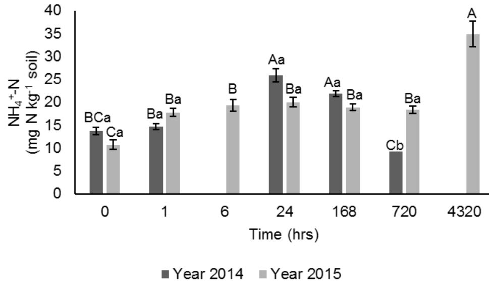
Fig. 2.7. Ammonium-N ( \text{NH}_4^+\text{-N} ) concentration in samples collected year 2014 and 2015 from prescribed fire, no-till, and conventionally tilled treatments pre- (0 hrs) and up to 4320 hrs (6 months) post-management of wheat residue. Different uppercase letters indicate significant differences within years over time. Different lowercase letters indicate significant differences within time between years. ( \alpha=0.05 )
