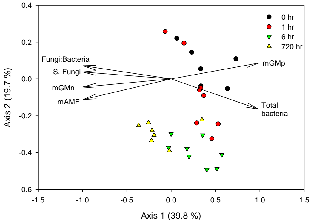
Fig. 2.20. Distance based redundancy analysis (db RDA) plot derived from fatty acid profiles from samples collected in corn stubble residue from prescribed fire treatment at pre- (0 hrs) and up to 720 hrs (30 days) post-management. Pre are black circles, 1 hr is red circles, 6 hrs are green triangles, and 720 hrs are gold triangles. Vectors in the bi-plot overlay were constructed from a matrix containing taxonomic groups. (mGMp = Gram positive bacteria; mGMn = Gram negative bacteria; mAMF = Arbuscular mycorrhizal fungi; S. Fungi = Saprophytic Fungi)
