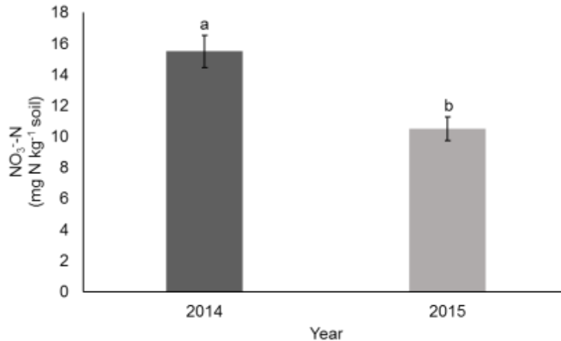
Fig. 2.5. Nitrate-N (NO 3 - -N) concentration in samples averaged over time from pre- (0 hrs) to 4320 hrs (6 months) post-prescribed fire and across prescribed fire, no-till, and conventionally tilled treatments in wheat residue. Different lowercase letters indicate significant differences within time and treatments between years. ( \alpha=0.05 )
