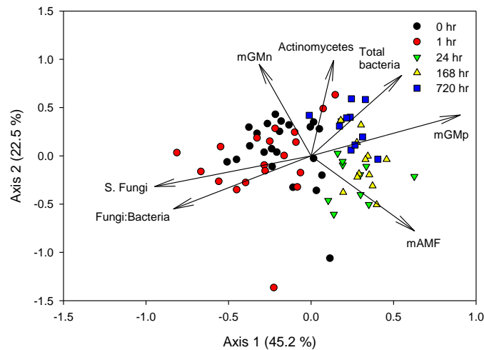
Fig. 2.17. Distance based redundancy analysis (db RDA) plot derived from fatty acid profiles from samples collected in 2014 wheat stubble residue from tilled, no-till, and prescribed fire treatments at pre- (0 hrs) and up to 720 hrs (30 days) post-management. Pre are black circles, 1 hr is red circles, 24 hrs are green triangles, 168 hrs are gold triangles, and 720 hrs are blue squares. Vectors in the bi-plot overlay were constructed from a matrix containing taxonomic groups. (mGMP = Gram positive bacteria; mGMn = Gram negative bacteria; mAMF = Arbuscular mycorrhizal fungi; S. Fungi = Saprophytic Fungi)
