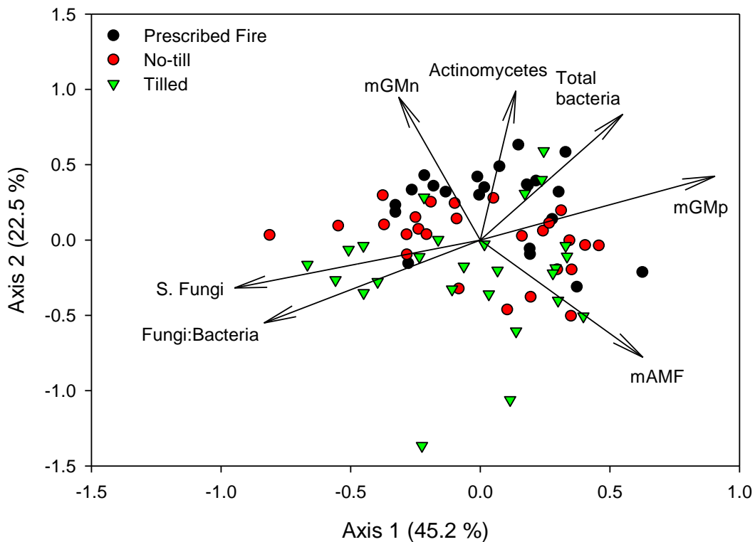
Fig. 2.16. Distance based redundancy analysis (db RDA) plot derived from fatty acid profiles from samples collected in 2014 wheat stubble residue under tilled (green triangles), no-till (red circles), and prescribed fire treatments (black circles). Vectors in the bi-plot overlay were constructed from a matrix containing taxonomic groups. (mGMp = Gram positive bacteria; mGMn = Gram negative bacteria; mAMF = Arbuscular mycorrhizal fungi; S. Fungi = Saprophytic Fungi)
